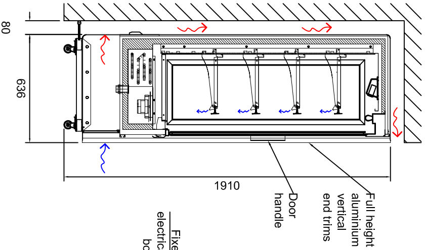
Side Elevation (Ventilation Space)
